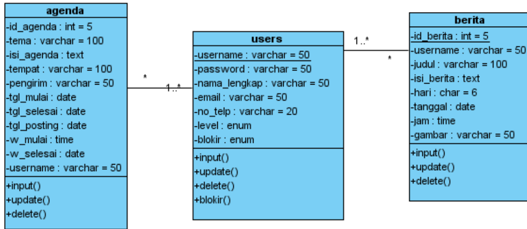
Gambar 4.16 Class diagram User
